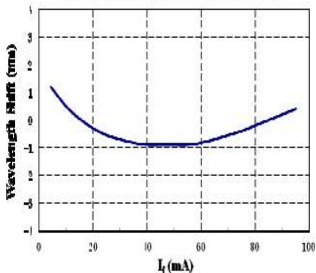
Wavelength Shift VS Forward Current
