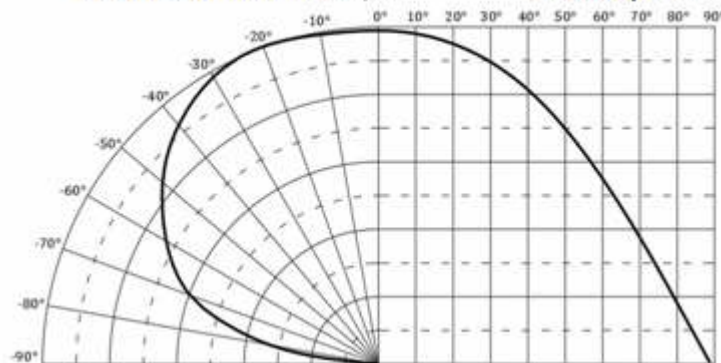
Radiation Characteristics \psi [°]
