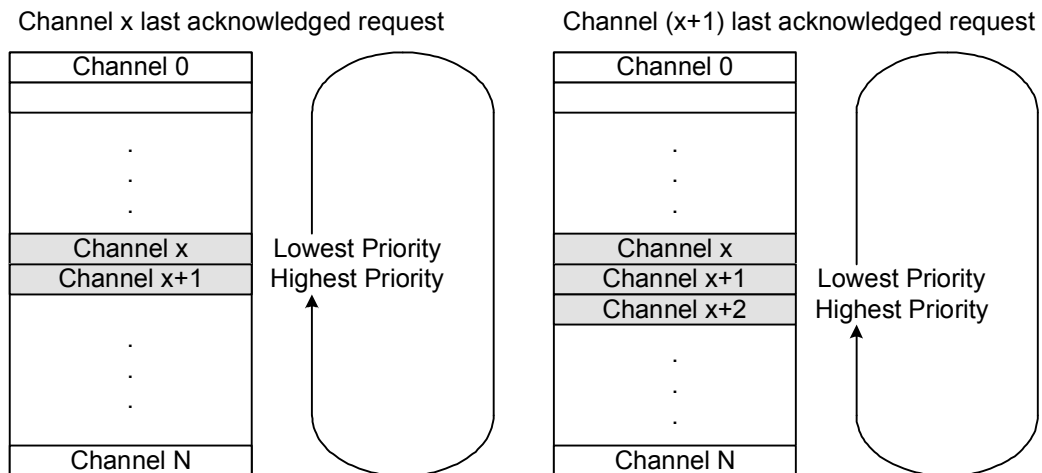
Figure 19-6. Round-Robin Scheduling
