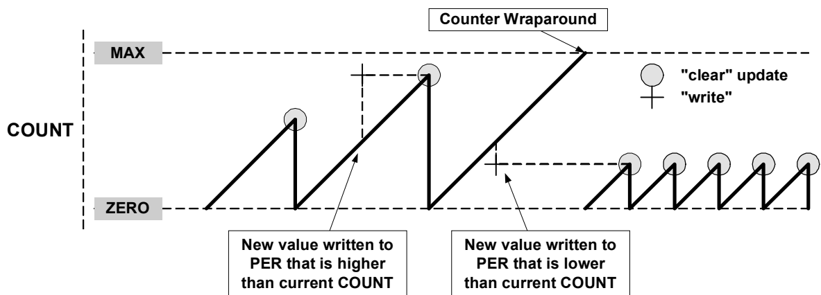
Figure 30-12. Unbuffered Single-Slope Up-Counting Operation
