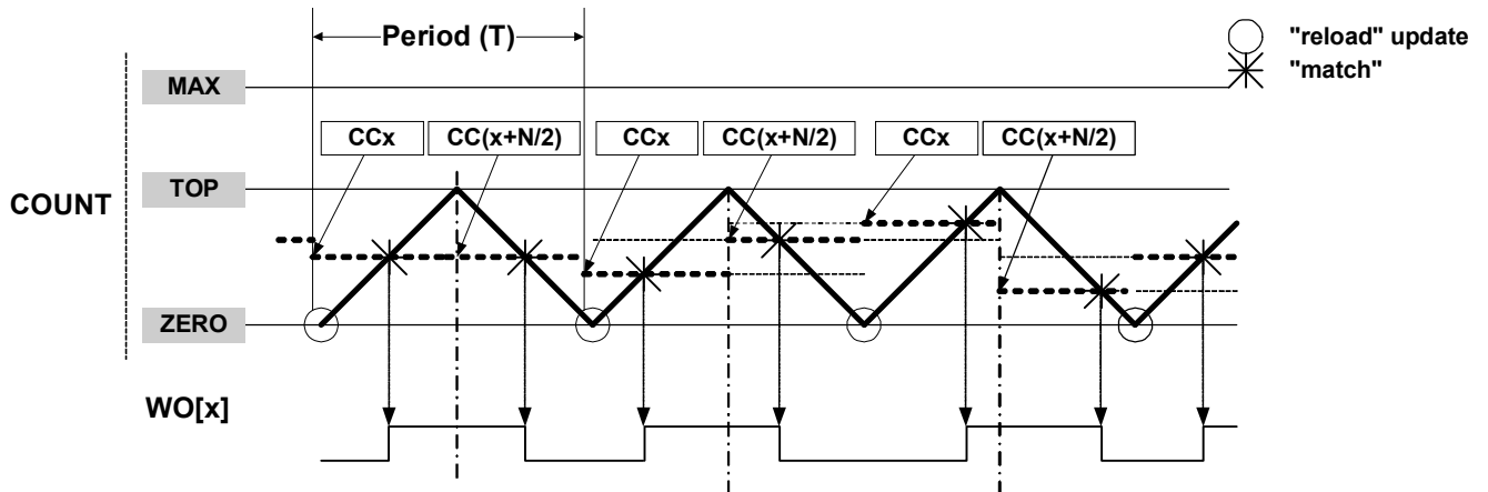
Figure 30-10. Dual-Slope Critical Pulse Width Modulation (N=CC_NUM)
