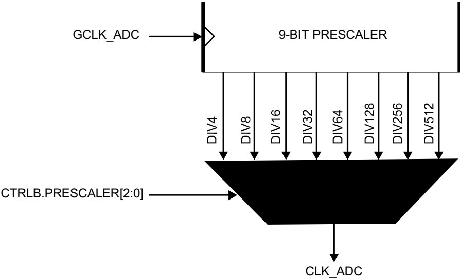
Figure 32-2. ADC Prescaler
