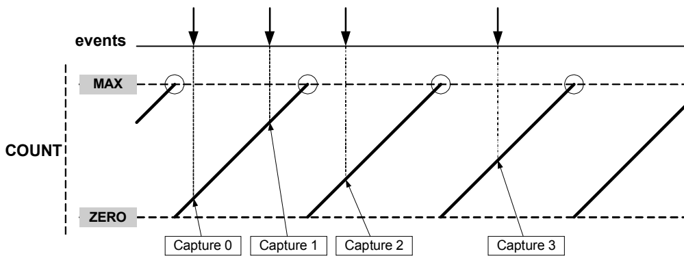
Figure 30-16.Input Capture Timing
