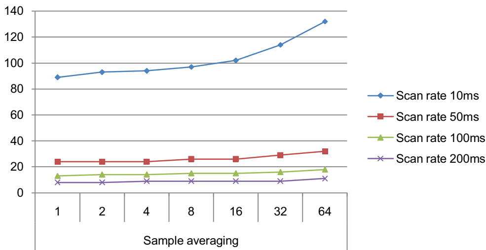
Figure 36-5. Power Consumption [ \mu A]
