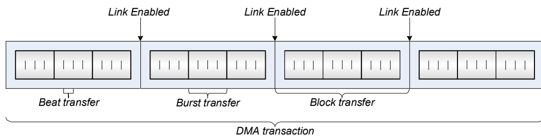
Figure 19-2. DMA Transfer Sizes
