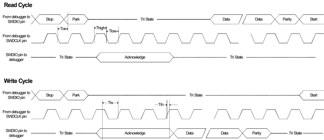
Figure 36-15.SWD Interface Signals
