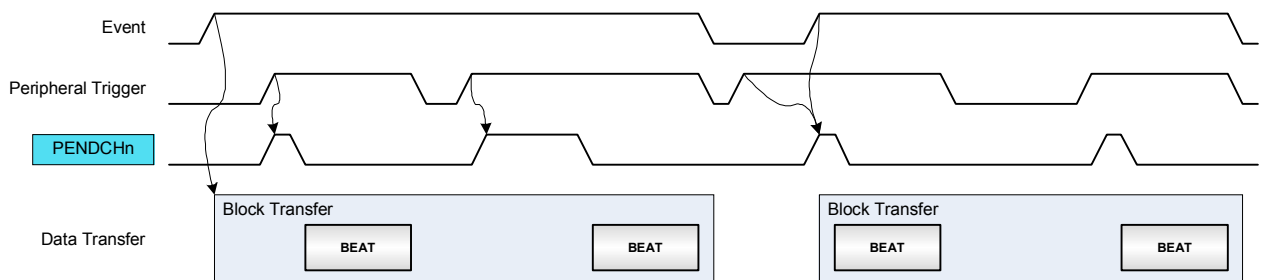
Figure 19-14. Conditional Block Transfer with Beat Peripheral Triggers
