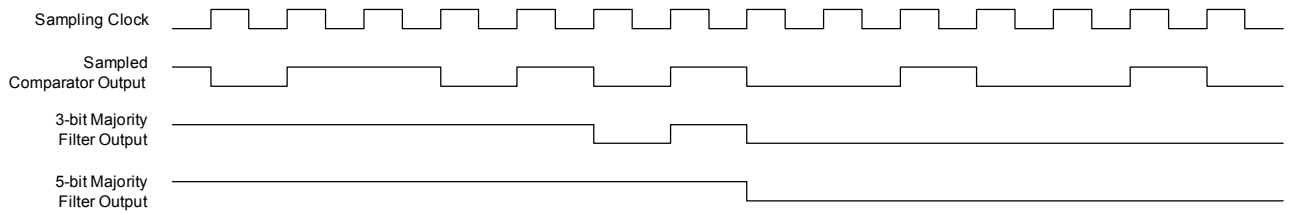
Figure 33-6. Continuous Mode Filtering
