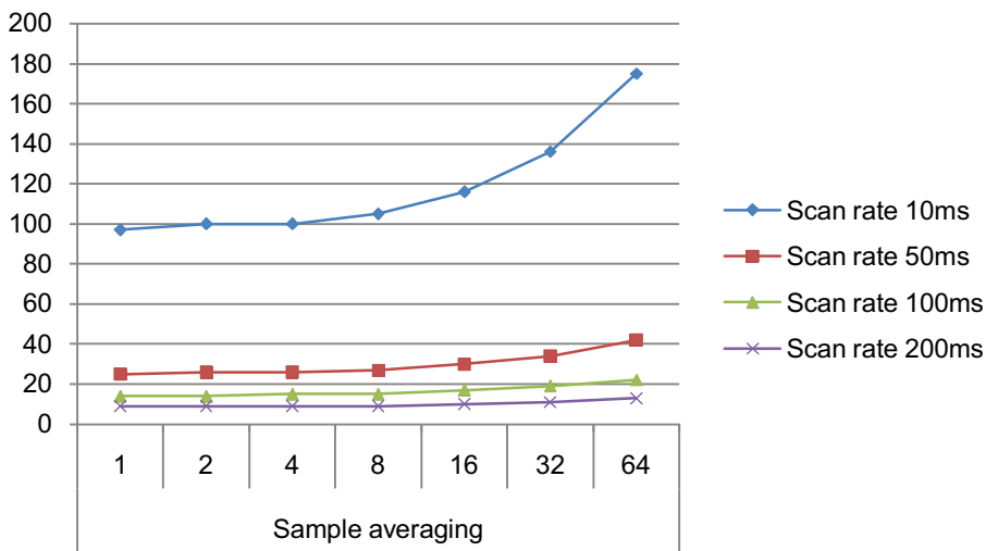
Figure 36-6. Power Consumption [ \mu A]
