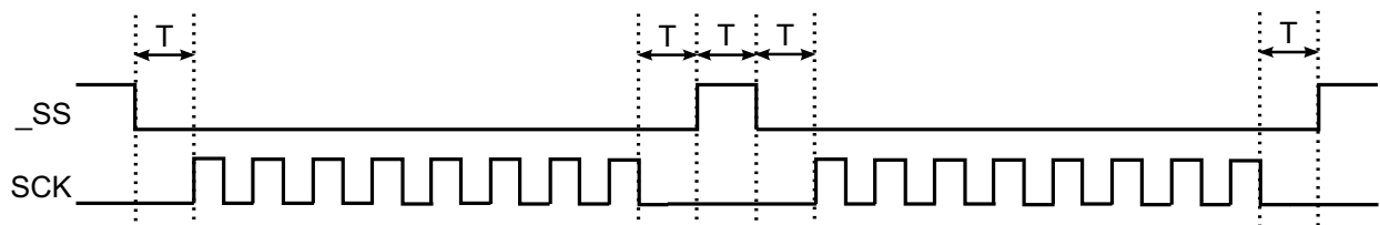
Figure 26-7. Hardware Controlled _SS
