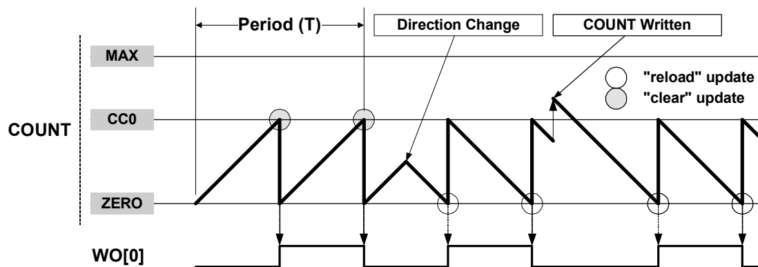
Figure 30-7. Match Frequency Operation
