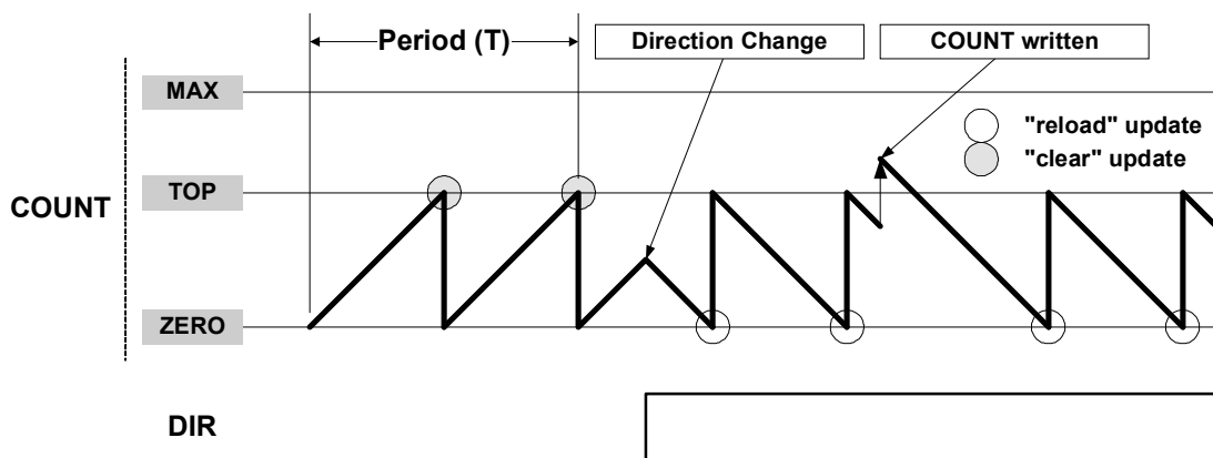
Figure 30-5. Counter Operation
