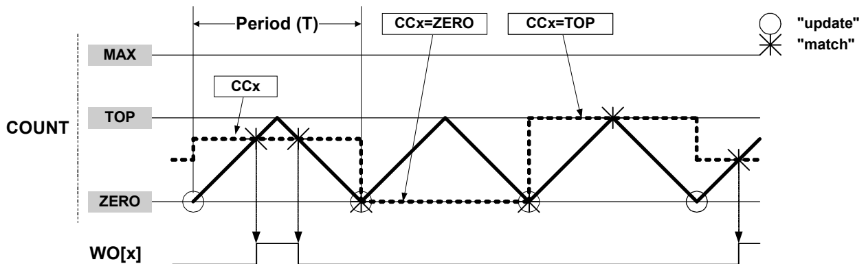
Figure 30-9. Dual-Slope Pulse Width Modulation
