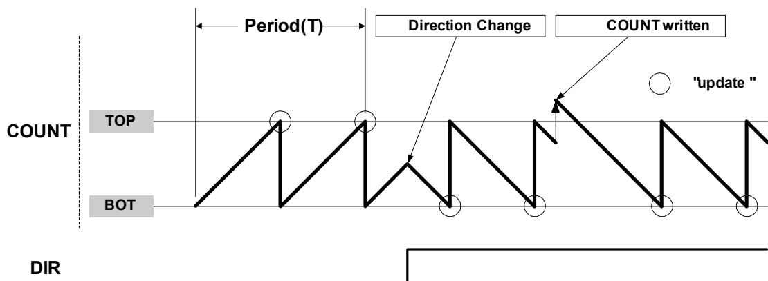
Figure 29-3. Counter Operation
