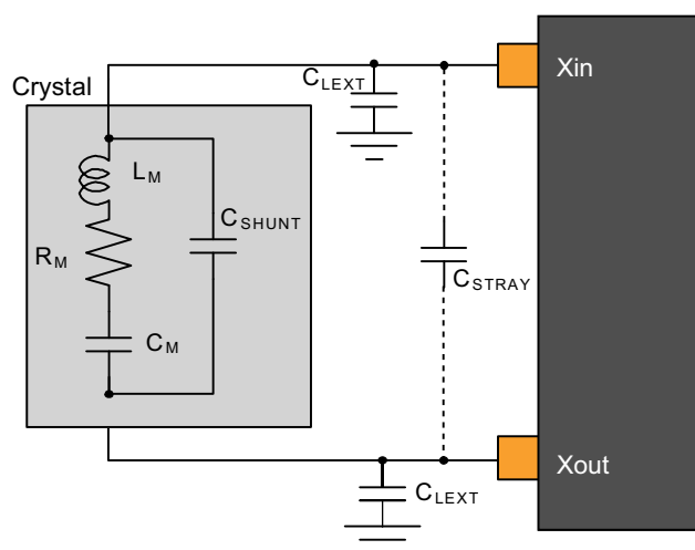
Figure 36-4. Oscillator Connection
