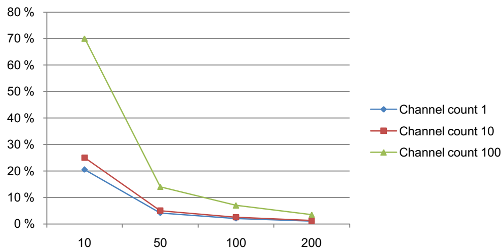
Figure 36-11.CPU Utilization
