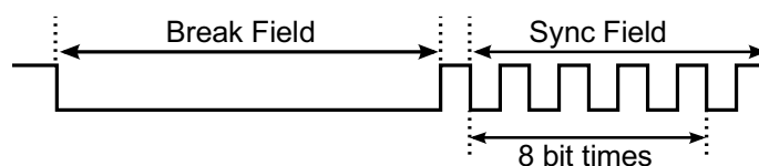
Figure 25-10. LIN Break and Sync Fields
