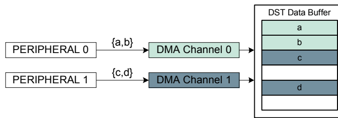
Figure 19-9. Destination Address Increment
