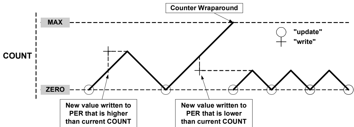
Figure 30-14. Unbuffered Dual-Slope Operation
