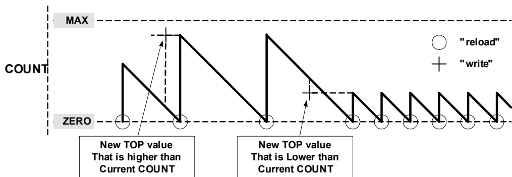
Figure 29-7. Changing the Top Value when Counting Down
