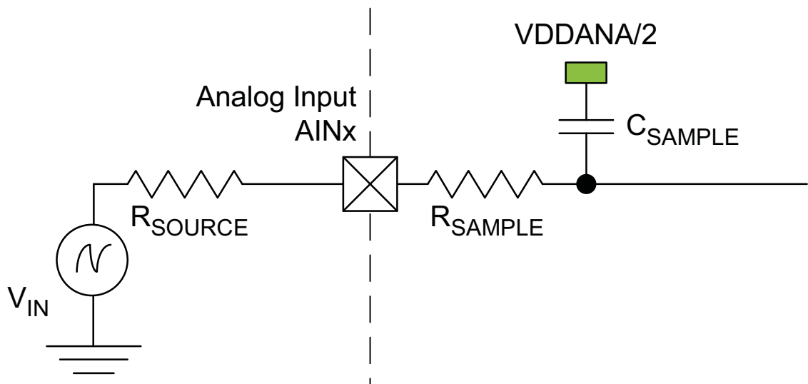
Figure 36-3. ADC Input
