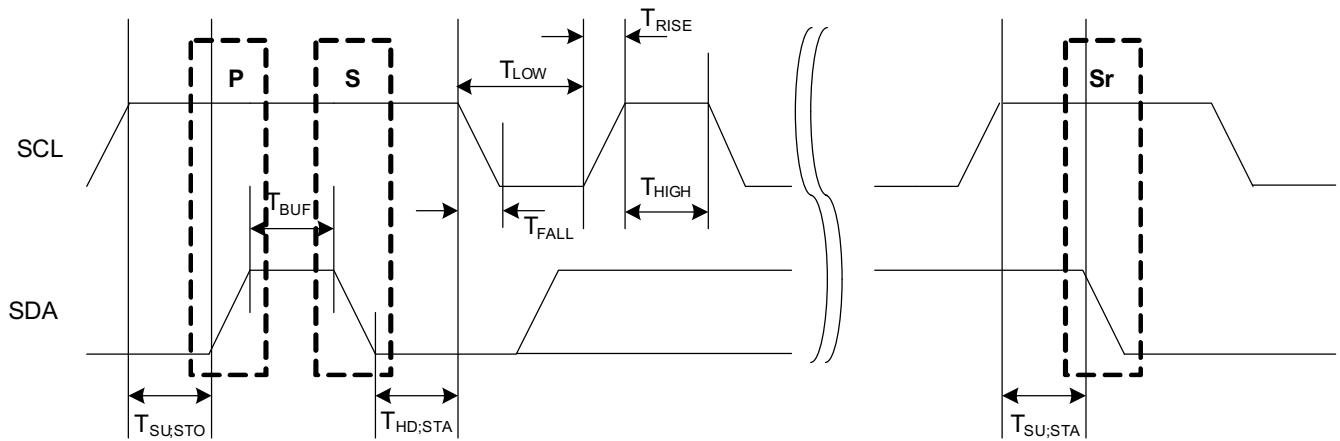
Figure 27-5. SCL Timing
