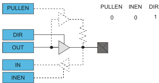
Figure 22-6. I/O Configuration - Totem-Pole Output with Disabled Input
