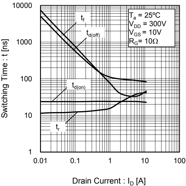
Fig.19 Switching Characteristics
