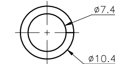
SPRING WASHER (1PCS)
