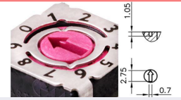
Arrow-shaped slot
