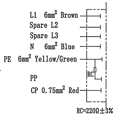
Wiring diagram
