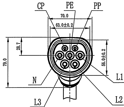
Wiring diagram
