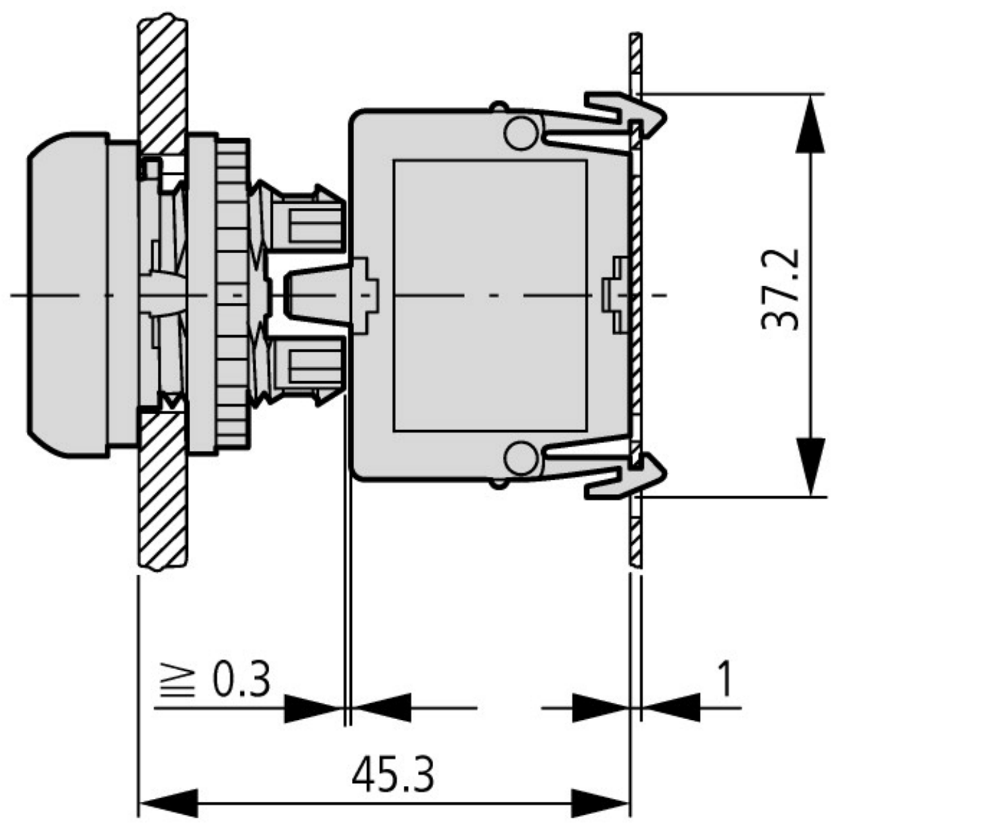
Pushbutton with M22-(C)K... Pushbutton with M22-(C) LED... + M22-XLED...
