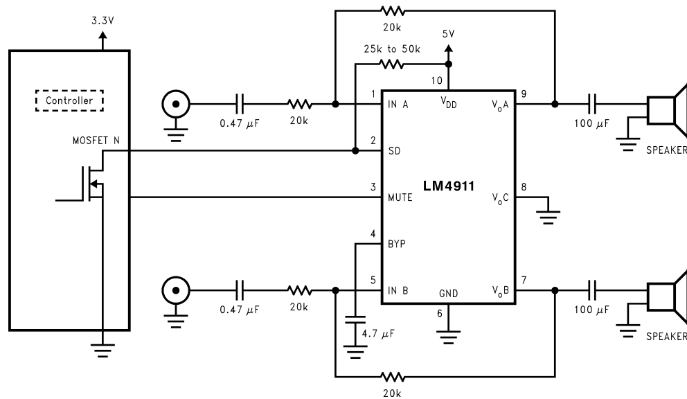
Figure 62. Recommended Circuit for Different Supply Turn-On Timing
