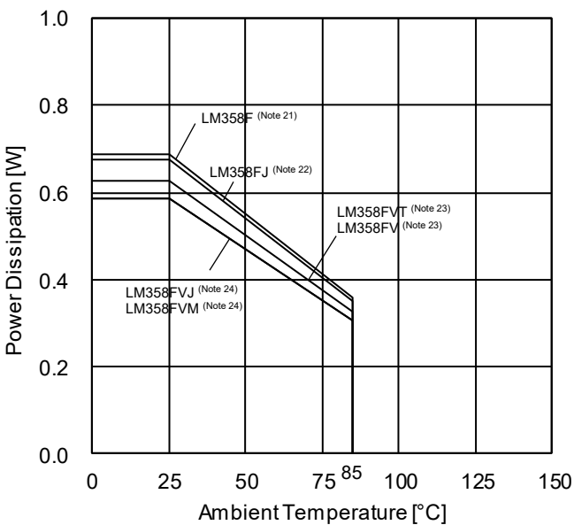
(c) LM358xxx*1
