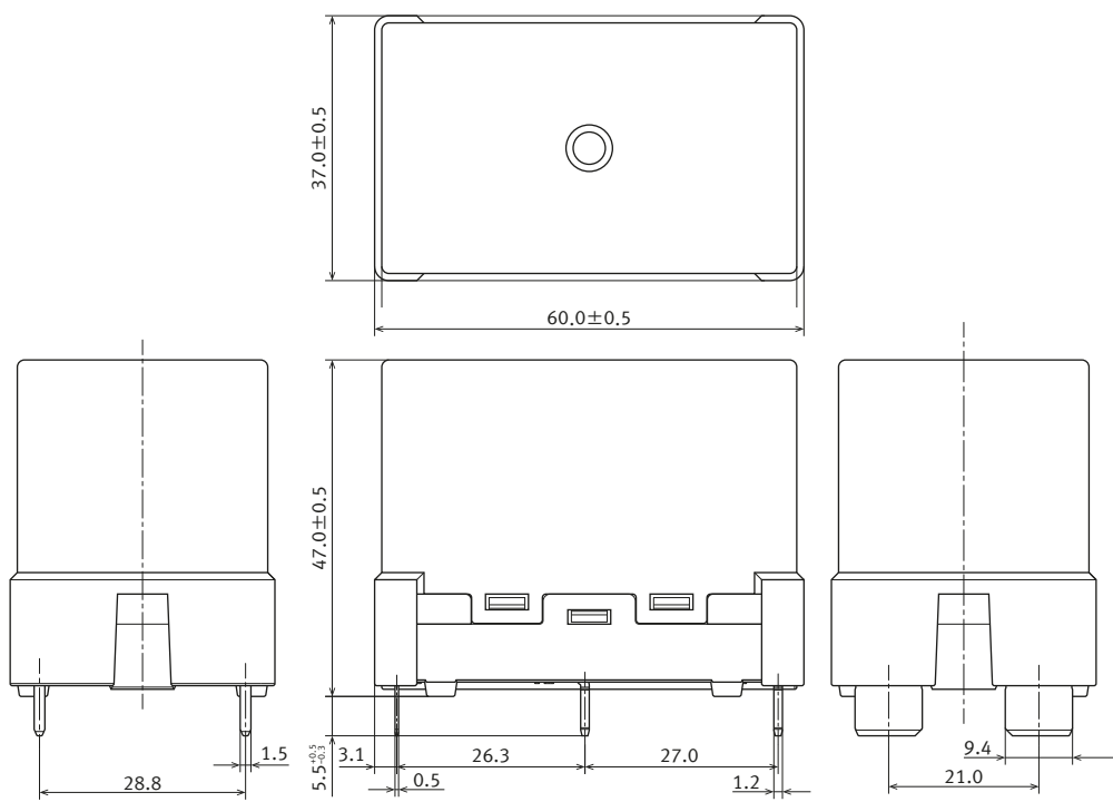
External dimensions
