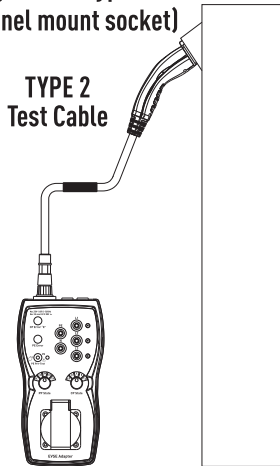
Connection of the test adapter to a charging station type 2 with panel mount socket outlet
