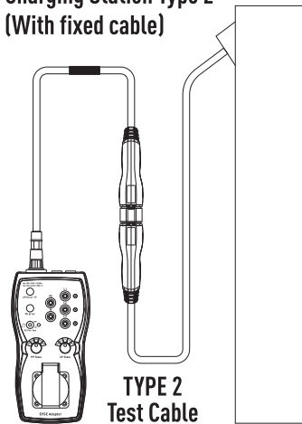
Connection of the test adapter to a charging station type 2 with fixed cable and vehicle connector
