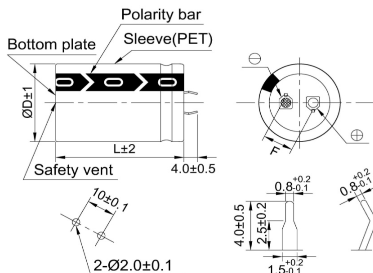
(PC board hole dimensions) (Terminal dimensions)
