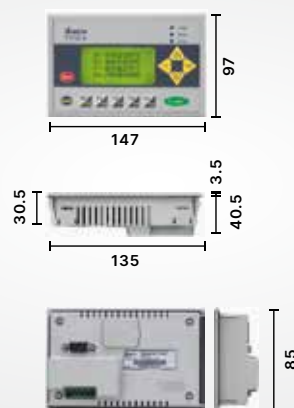
TP04G-BL-C
