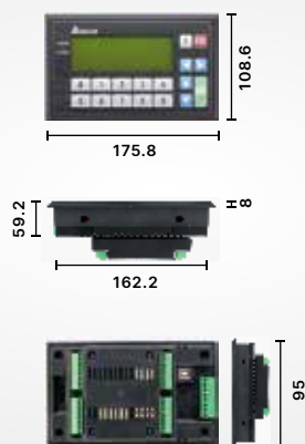
TP04P-Series
