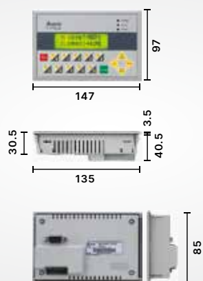
TP04G-AL-C/TP04G-AL2
