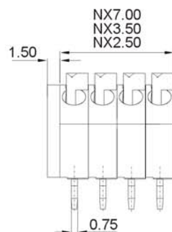
W/O COVER VIEW
