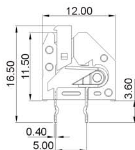
W/O COVER VIEW
