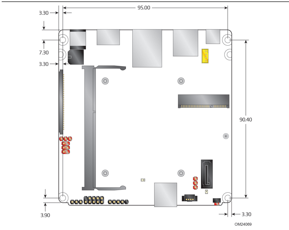
Figure 21. Board Dimensions
