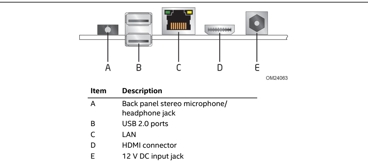
Figure 11. Back Panel Connectors
