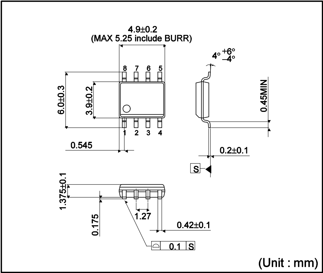
SOP-J8
