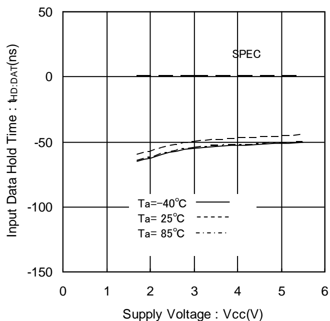
Figure 22. Input Data Hold Time vs Supply Voltage (LOW)
