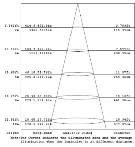
Lux Diagram
