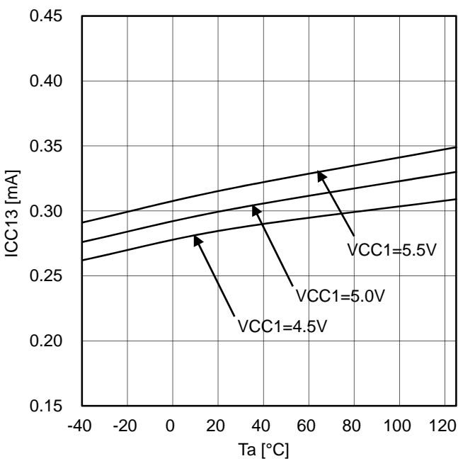
Figure 14. Input Side Circuit Current 3 (at INA=20kHz , Duty=50%)
