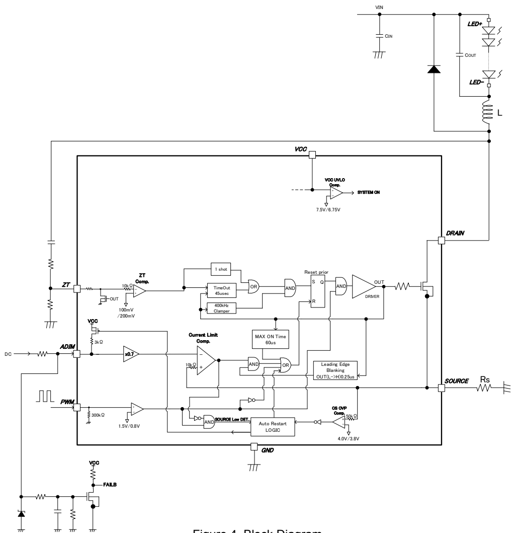
Figure 4. Block Diagram
