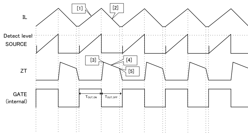
Figure 7. Dimming Waveform
