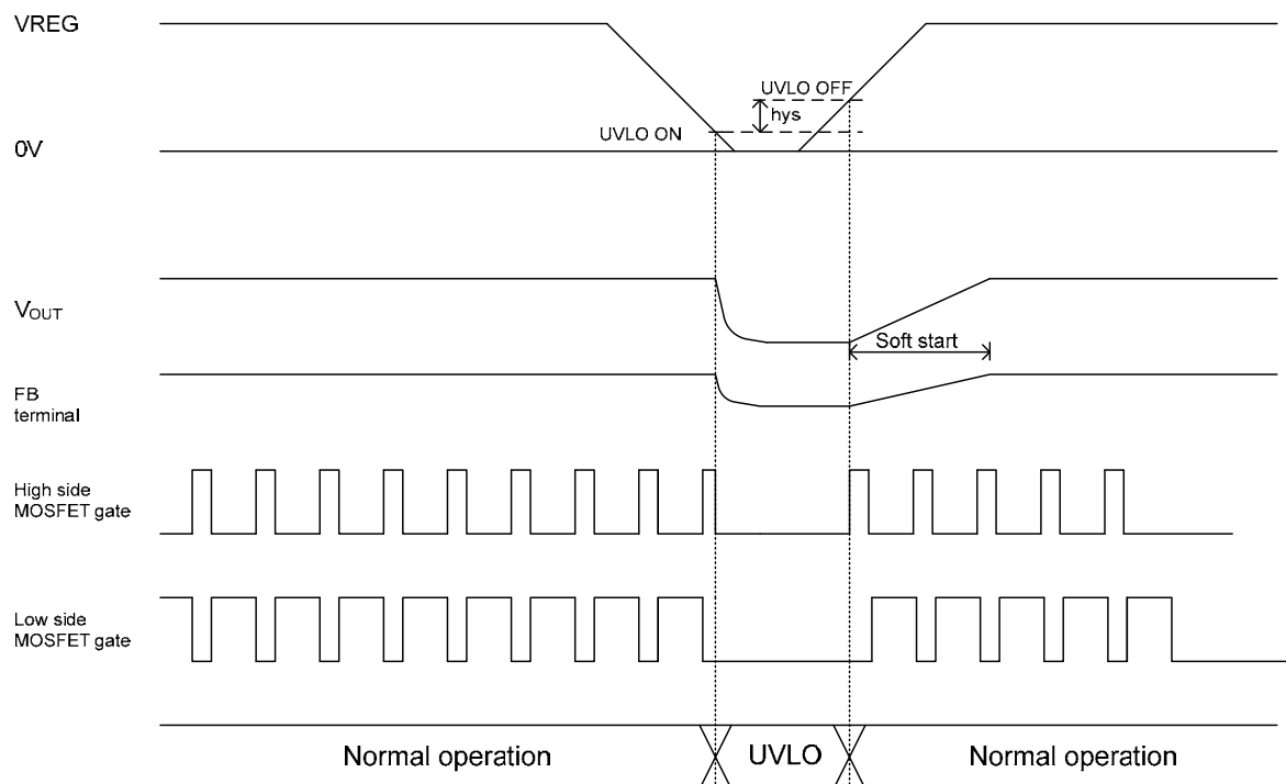
Figure 27. UVLO Timing Chart
