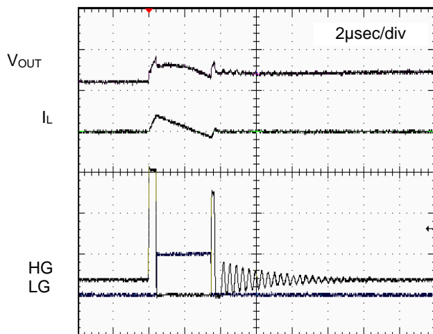
Figure 13. SLLM™ Mode ( I_{OUT}=0A )
