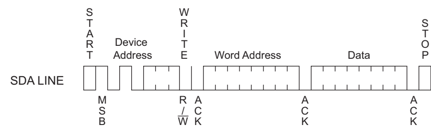
Figure 8-2. Byte Write
