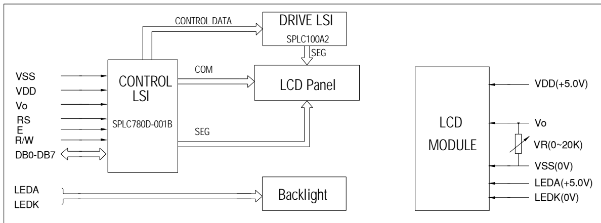
Figure 2. Block diagram
