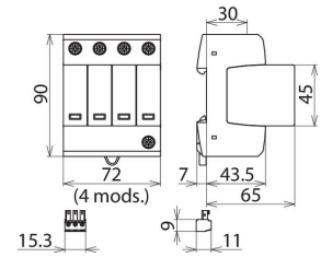
Dimension drawing VT2 M TT 320 FM
