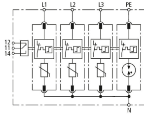
Basic circuit diagram VT2 M TT 320 FM
