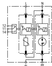
Basic circuit diagram DG M TT 2P 320 FM
