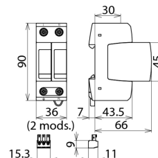
Dimension drawing DG M TT 2P 320 FM
