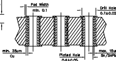
RECOMMENDED HOLE SPECIFICATIONS SECTION A-A SCALE 6 : 1
