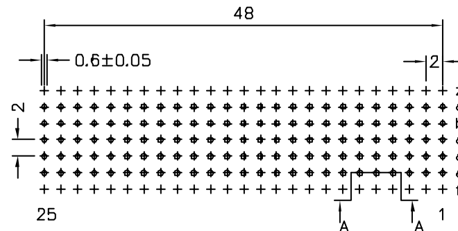
RECOMMENDED PCB HOLE LAYOUT COMPONENT SIDE SCALE 1.5 : 1
