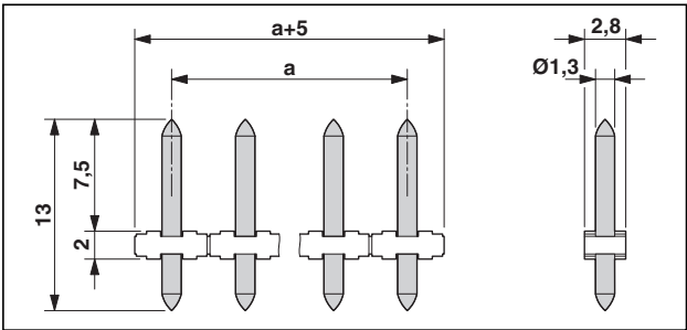
Figure 25 Dimensions PST 1,3/ ...-5,0
