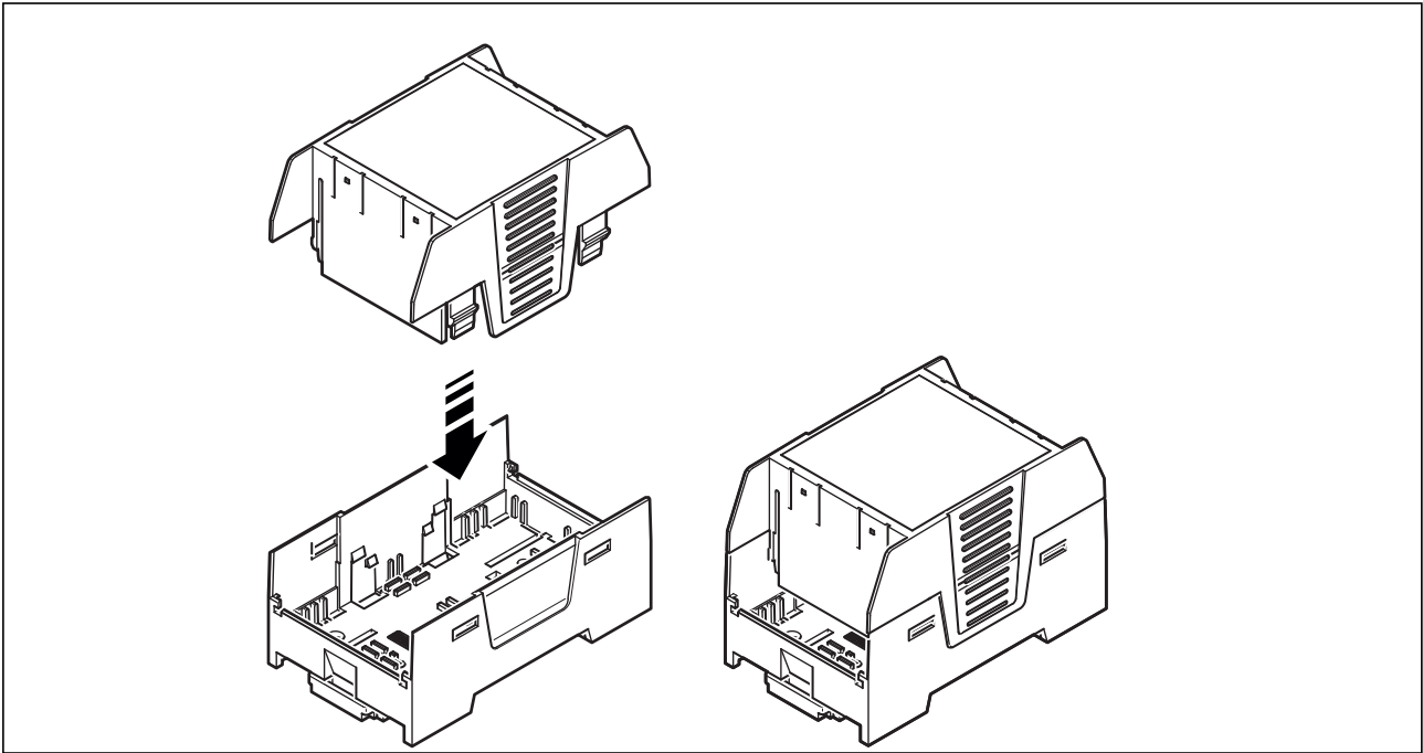
Figure 33 Snapping on the housing cover
