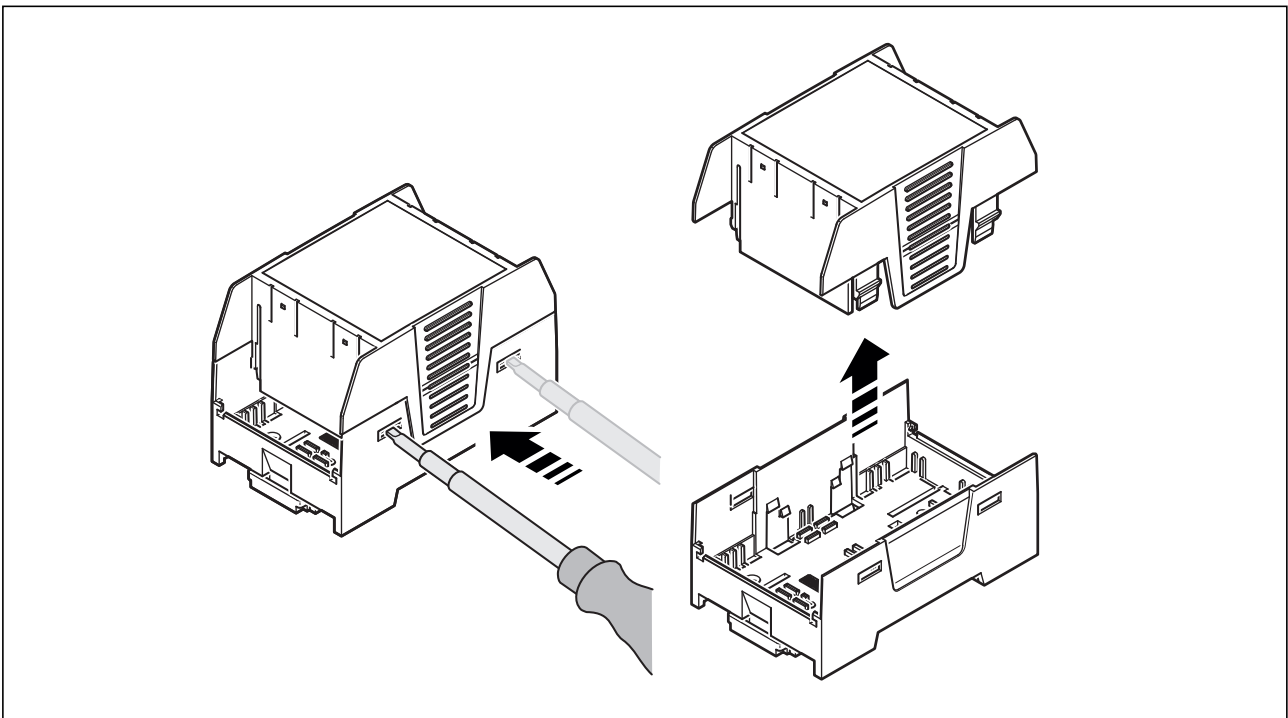
Figure 34 Releasing the housing cover
