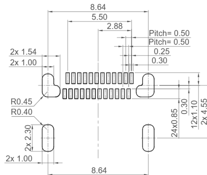
Recommended Solder mask Thickness = 0.12mm Tolerance: \pm 0.05\text{mm}
