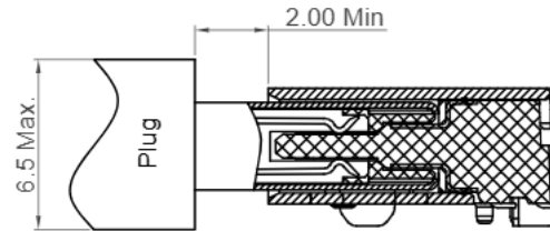
Plug and Receptacle Mating View
