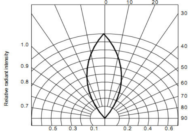
Fig.6 Radiation diagram
