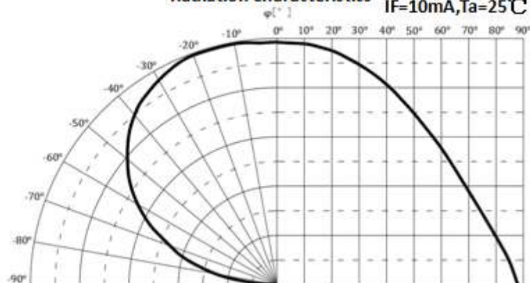
Radiation Characteristics
