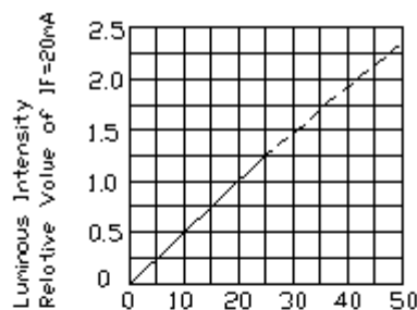
Ir-Forward Current (mA) LUMINOUS INTENSITY Vs. FORWARD CURRENT
