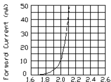
Forward Voltage (V) FORWARD CURRENT Vs. FORWARD VOLTAGE
