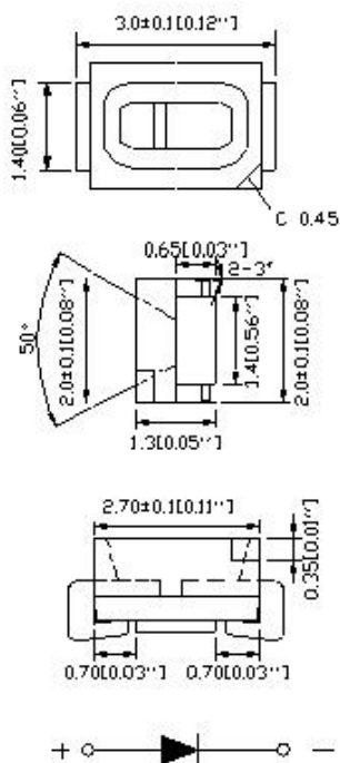
Package outlines
