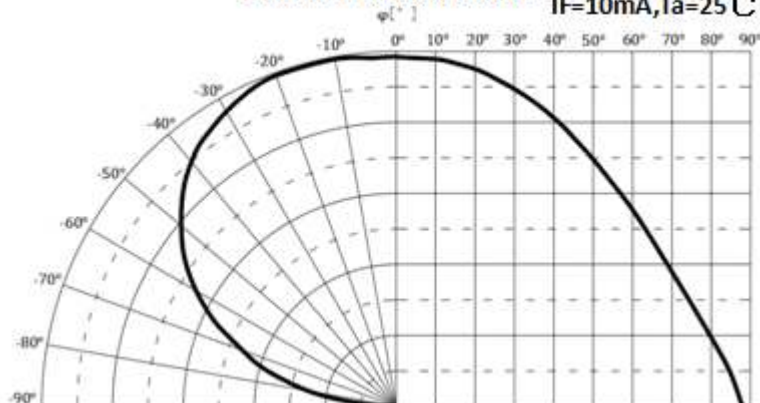
Radiation Characteristics I_F = 10\text{mA}, T_a = 25^\circ\text{C}
