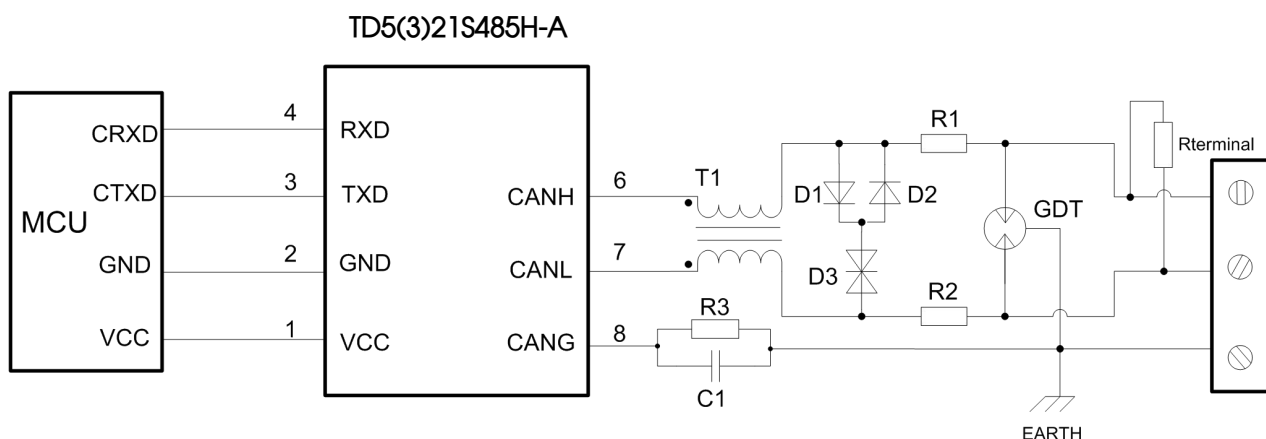
Fig. 2: Port protection circuit for harsh environments
