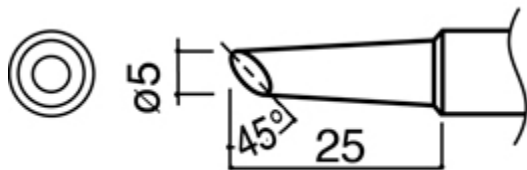
A1048 Shape-3C
