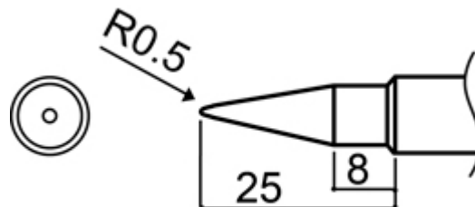
A1047 Shape-B
