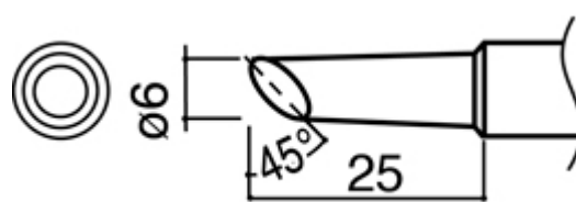
A1049 Shape-4C
