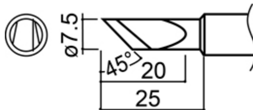
A1053 Shape-K
