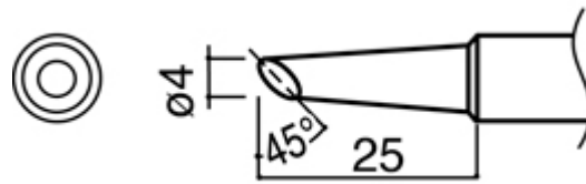
A1049 Shape-4C
