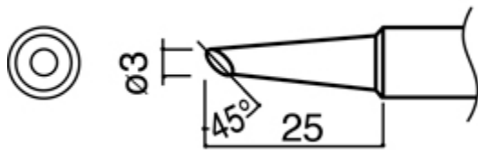
A1048 Shape-3C
