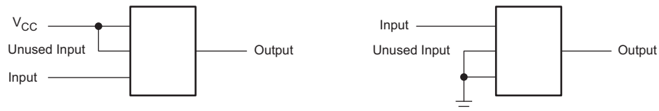
Figure 9. Proper Multi-Gate Input Termination Diagram
