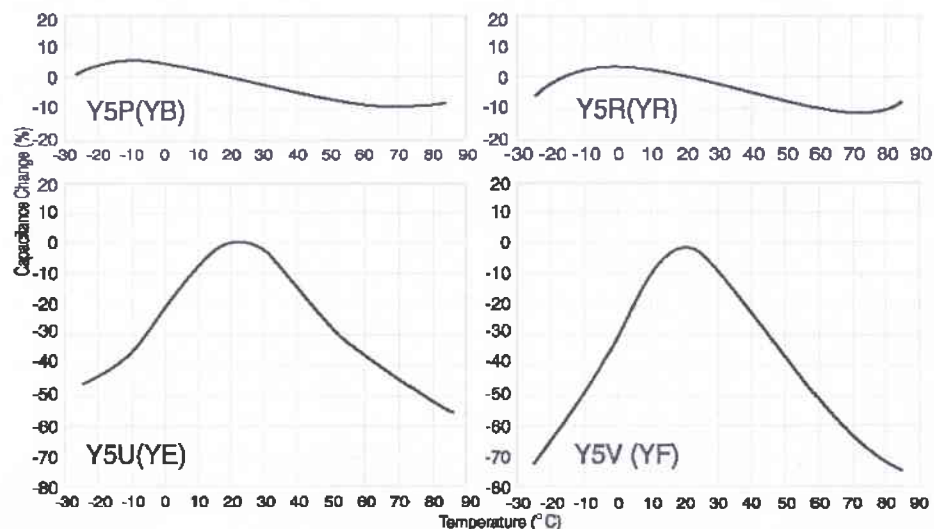
Capacitance Temperature Characteristics
