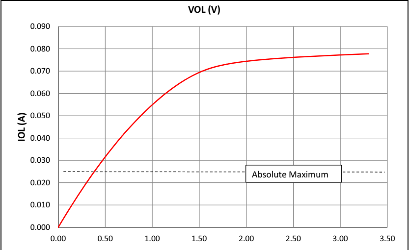
FIGURE 39-4: V_{OL} – 8x DRIVER PINS
