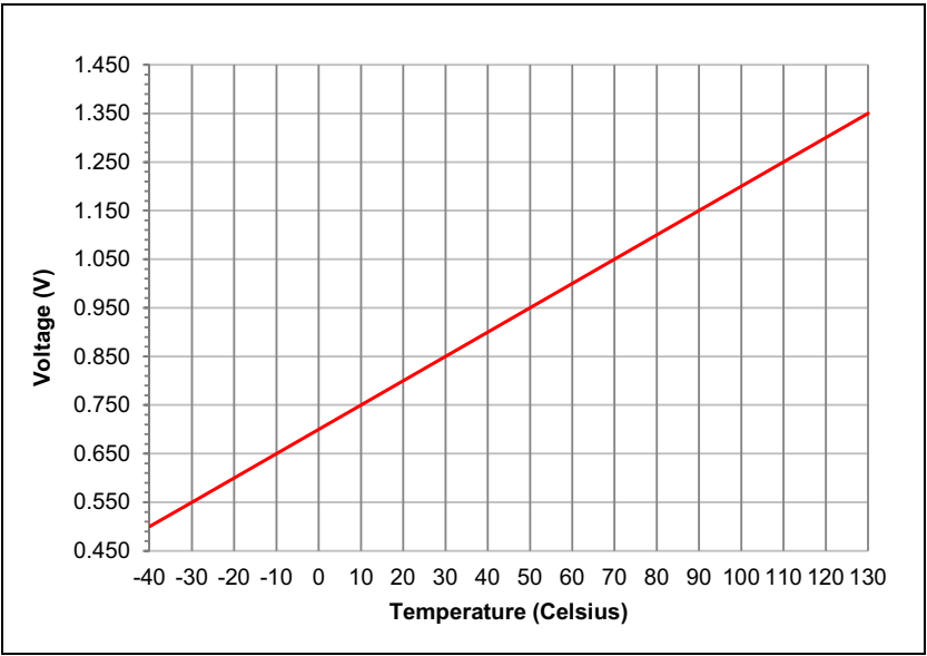
FIGURE 39-7: TYPICAL TEMPERATURE SENSOR VOLTAGE
