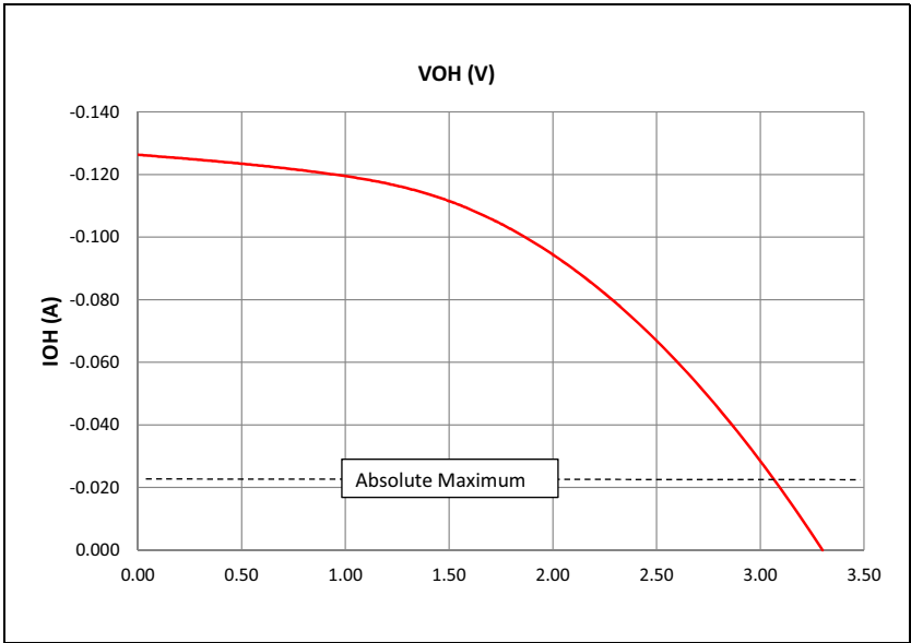
FIGURE 39-5: V_{OH} – 12x DRIVER PINS
