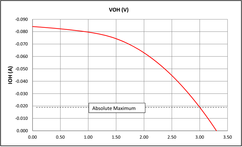
FIGURE 39-3: V_{OH} – 8x DRIVER PINS
