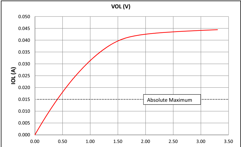
FIGURE 39-2: V_{OL} – 4x DRIVER PINS
