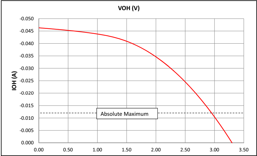
FIGURE 39-1: V_{OH} – 4x DRIVER PINS
