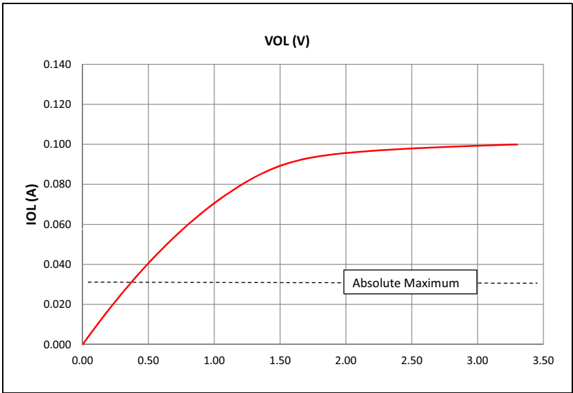
FIGURE 39-6: V_{OL} – 12x DRIVER PINS
