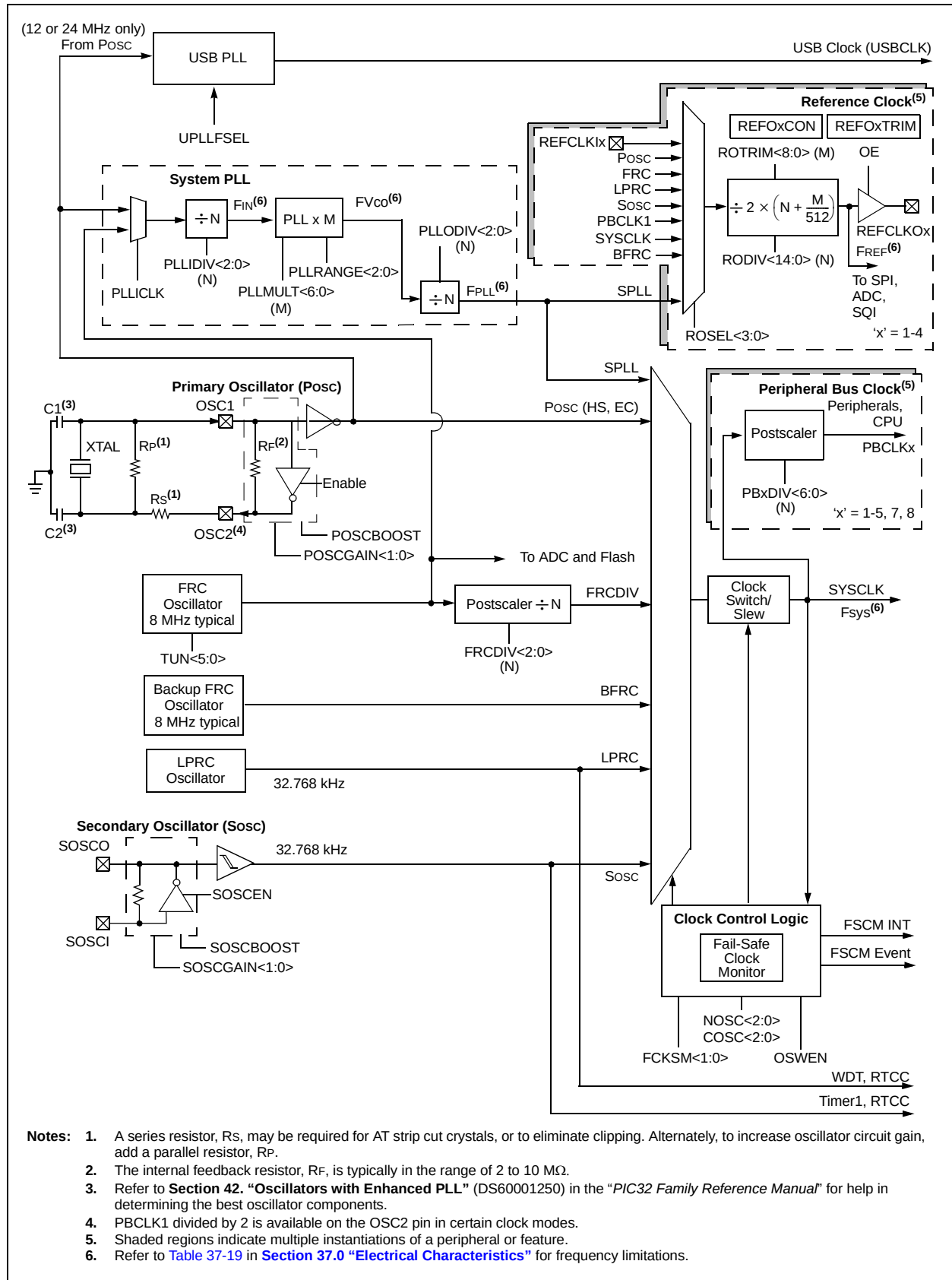
FIGURE 8-1: PIC32MZ EF FAMILY OSCILLATOR DIAGRAM
