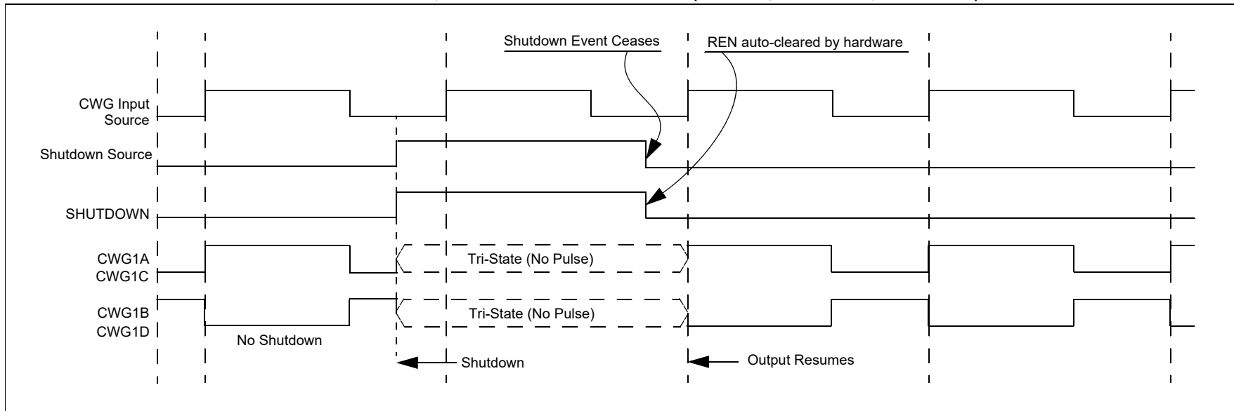
FIGURE 30-14: SHUTDOWN FUNCTIONALITY, AUTO-RESTART ENABLED (REN = 1, LSAC = 01, LSBSD = 01)
