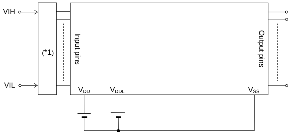
Measuring circuit 5
