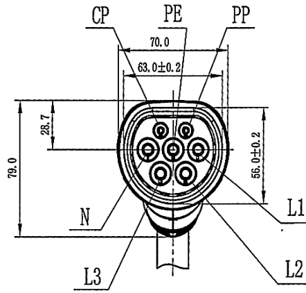
Wiring diagram
