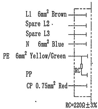
Wiring diagram
