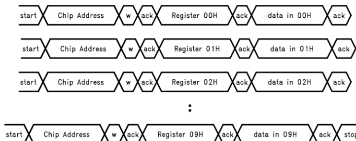
Figure 8. Programming With Auto Increment Disabled (in WRITE Mode)
