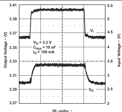
Figure 8-11. Line Transient Response for Legacy Chip
