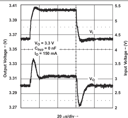
Figure 8-9. Line Transient Response for Legacy Chip
