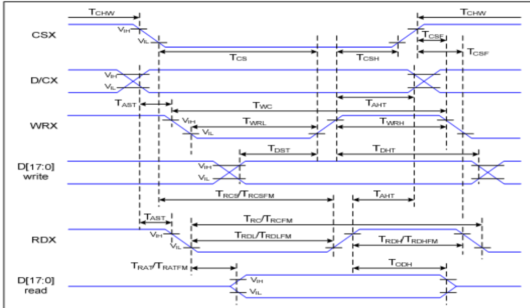
Fig. 8.1.1 Parallel interface timing characteristics (8080 series MCU interface)
