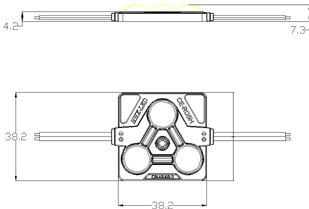
FIG. dimension of HHX-M36363-28T/36363-56T
