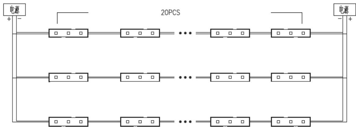
HHX-74123FT-56Tcircuit layout
