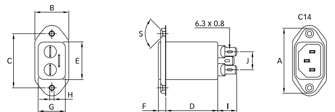
FN 9222 U
