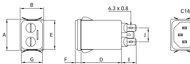
FN 9222 S
