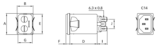
FN 9222 S1
