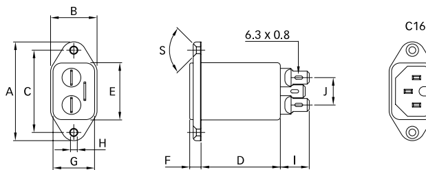
FN 9222-HI
