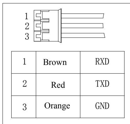
RS232 Communication Cable
