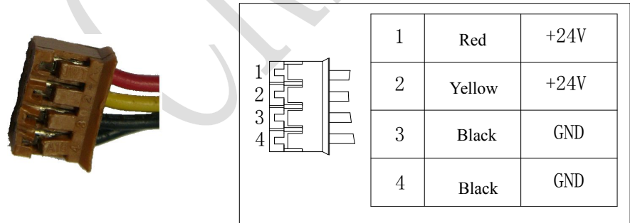
Picture2 4 PIN Power cable
