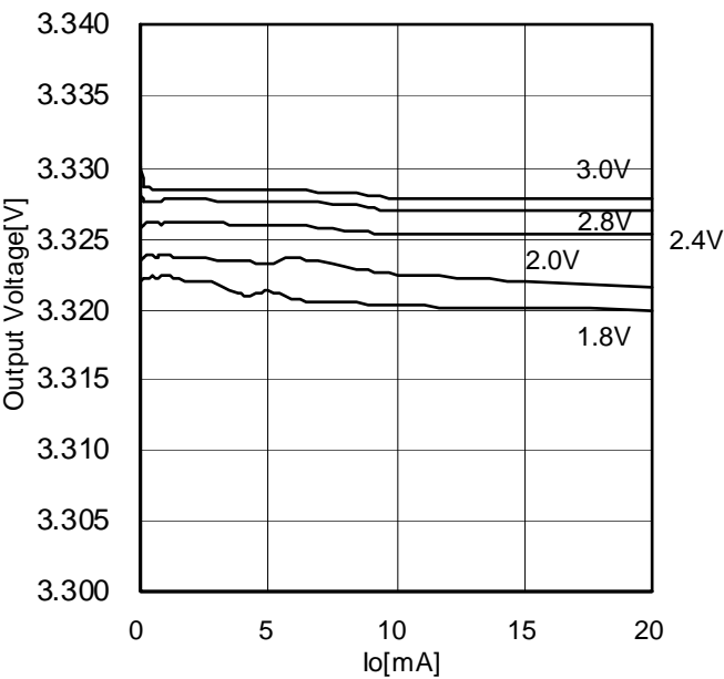
Figure 13. Load-Regulation[Ta=-85°C]
