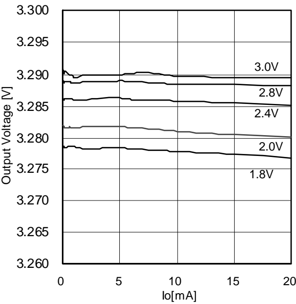
Figure 11. Load-Regulation[Ta=-30°C]
