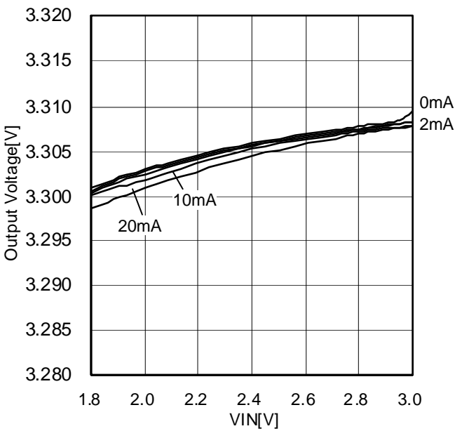
Figure 15. Line-Regulation [Ta=25°C]
