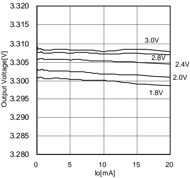
Figure 12. Load-Regulation [Ta=25°C]
