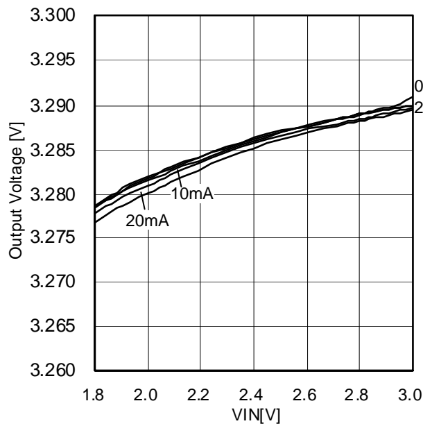
Figure 14. Line-Regulation[Ta=-30°C]
