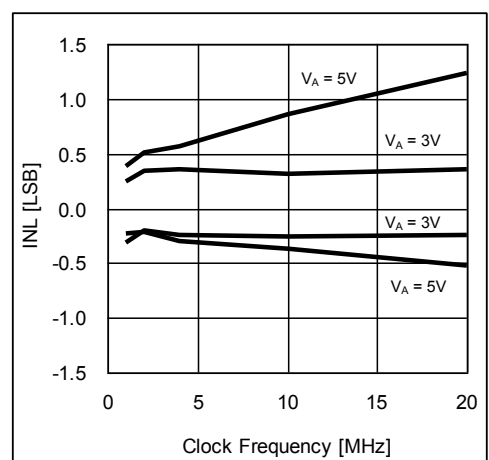
Figure 11. INL vs CLOCK FREQUENCY
