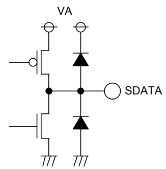
Figure 26. Equivalent Digital Output Circuit
